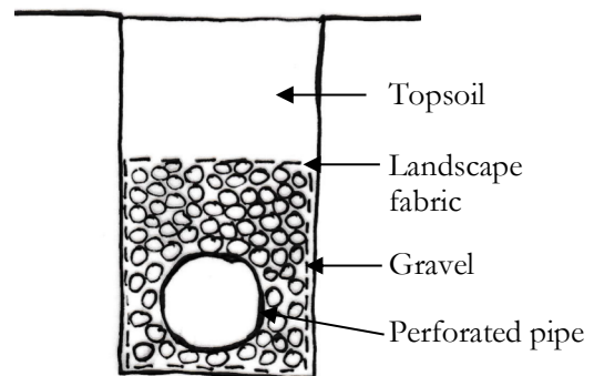
Piped drainage
